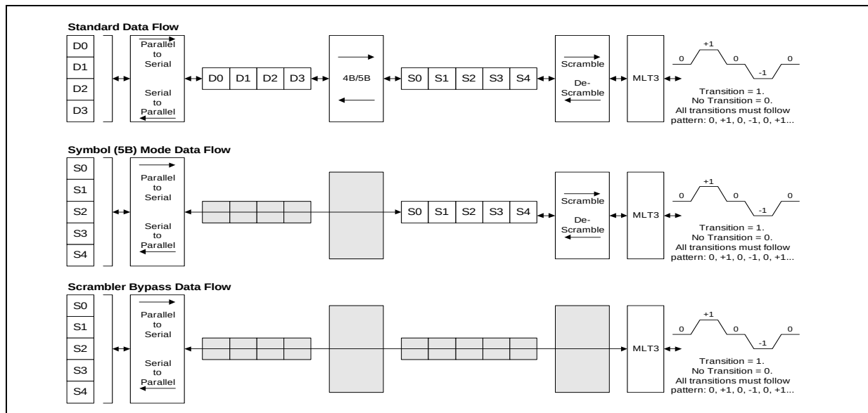
Figure 14. 100BASE-TX Data Flow
